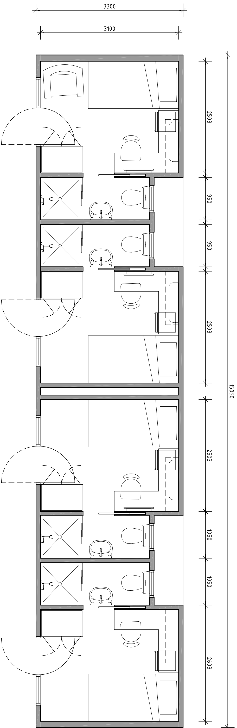
4 SINGLE PERSON QUARTERS 15060 X 3300
